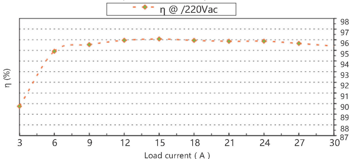
Output Current-Efficiency Curve
